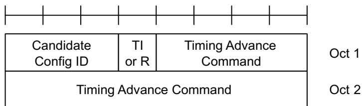
Figure 6.1.3.4b-1: LTM Candidate Timing Advance Command MAC CE
